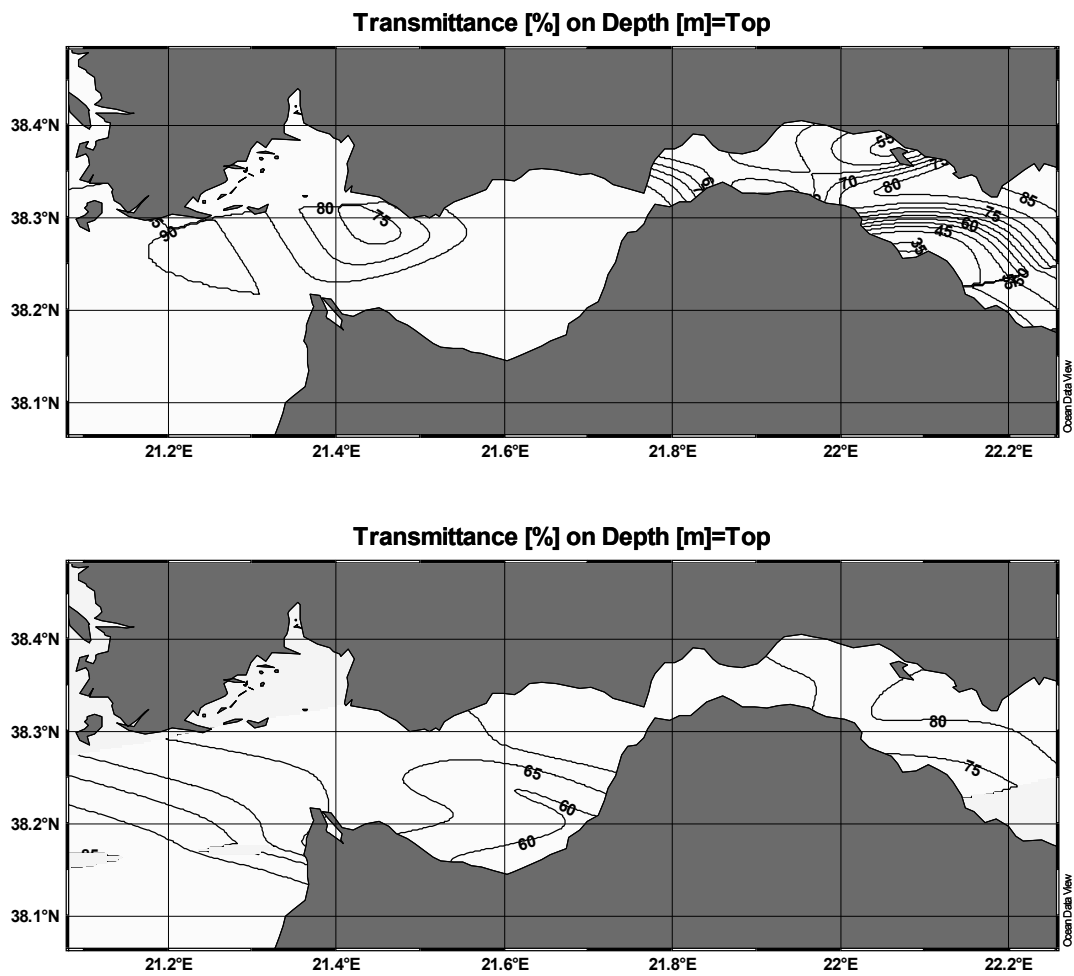
Figure 3. Surface distribution of transmittance (%) in: (a) late spring (June) and (b) late autumn (December).
