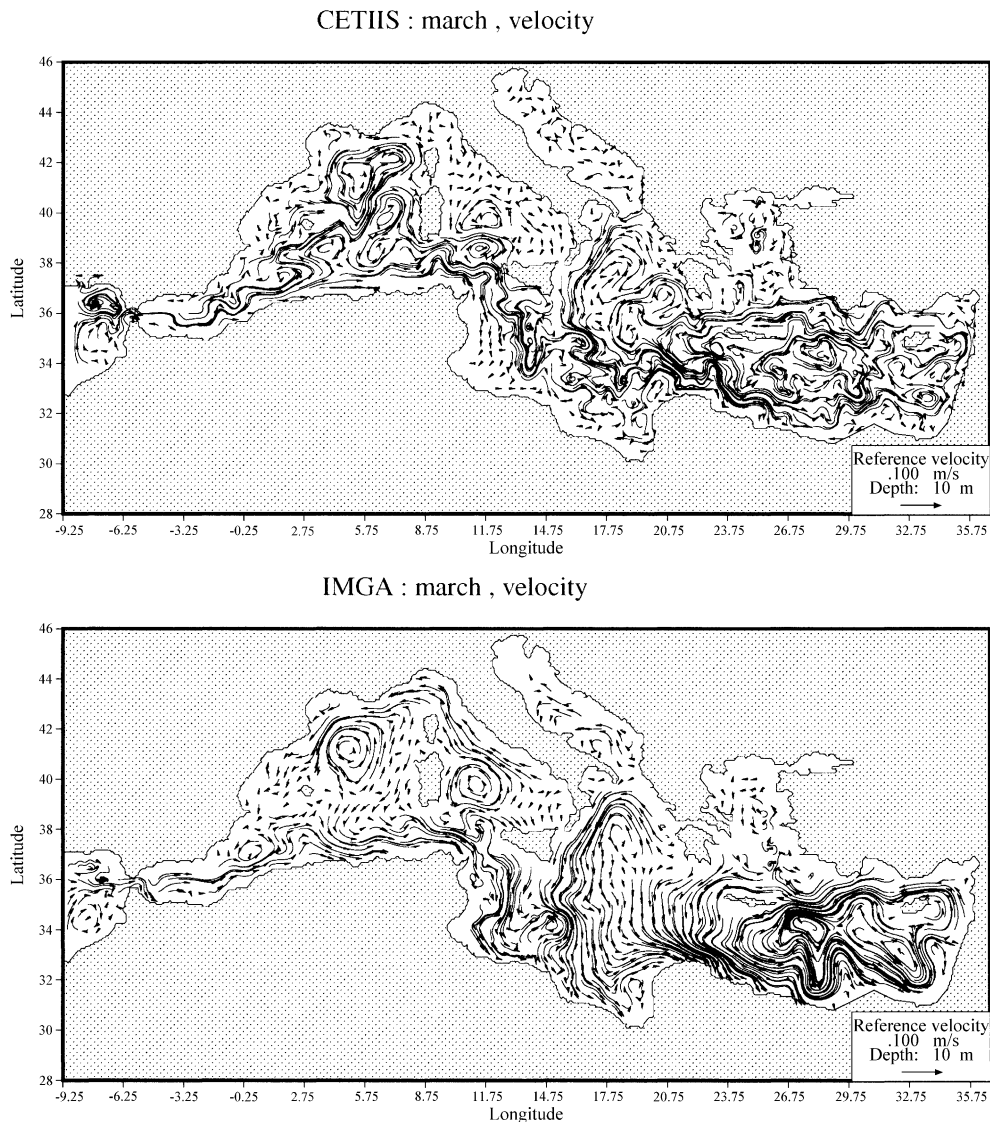
Fig. 15. Velocity fields March Average, experiment II.
