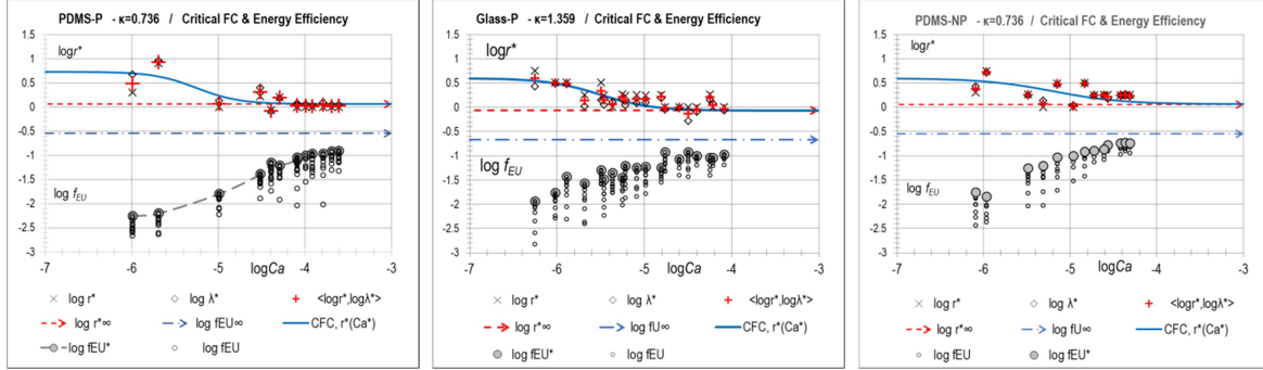
Fig. 8. Energy efficiency values \{r_j, f_{EU,i}\} , \circ , and detected maximum values \{Ca_i, f_{EU,i}^*\} , \bullet , for the three systems examined in the study (PDMS-P, Glass-P and PDMS-NP). The corresponding critical flow rate ratio values, \{Ca_i, r_i^*\} , \times , and mobility ratio values, \{Ca_i, \lambda_i^*\} , \diamond , define the so-called Critical Flow Conditions; upright cross markers in red, + , indicate the mean of the flow rate ratio and mobility ratio values, \hat{r}^* , Eq. (21).
