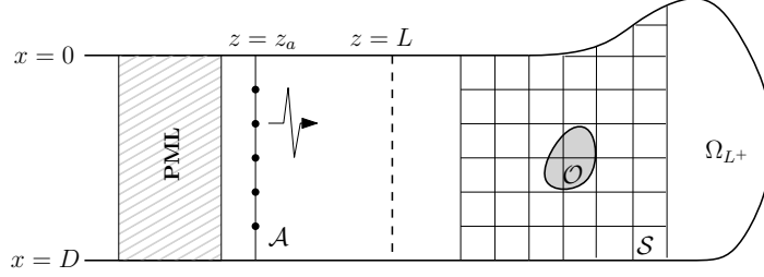
Fig. 12: Sketch of a waveguide that is truncated near the array with a PML.
