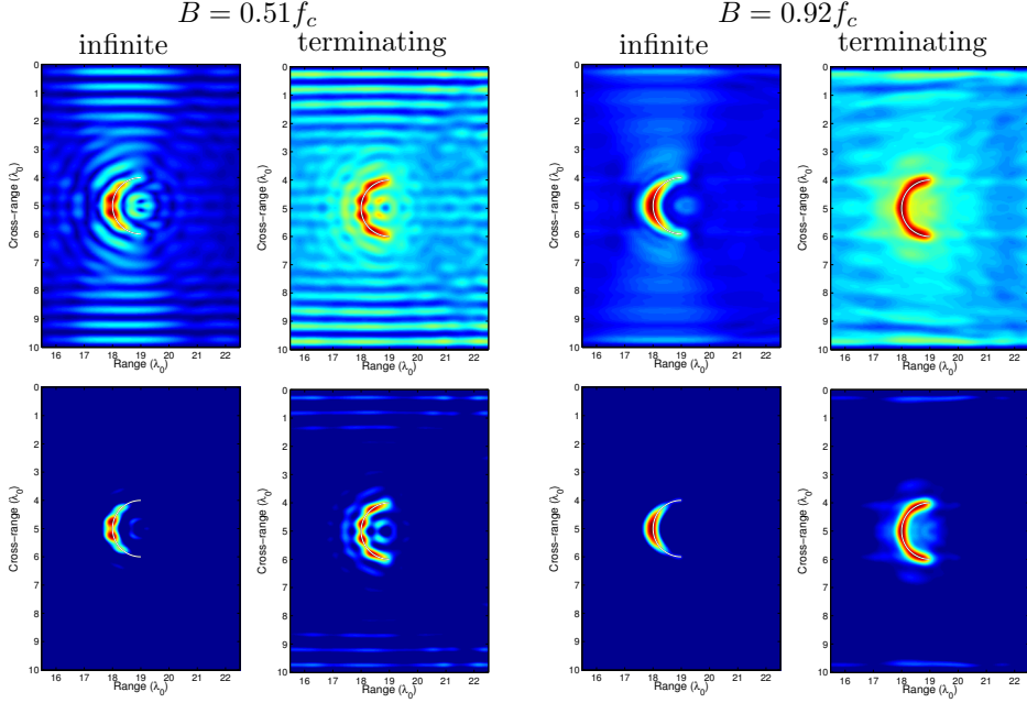
Fig. 11: Multiple frequency imaging with \mathcal{I}^* of a semicircular reflector centered at (z^*, x^*) = (19, 5)\lambda_0 . Specifically, f \in [f_c - B/2, f_c + B/2] with k_c = 0.975k_0 , k_0 = \pi/10 . For the first two columns the bandwidth is equal to B = 0.51f_c , while a larger bandwidth B = 0.92f_c is used for the two columns on the right. The images shown in the first and in the third column correspond to the open-ended waveguide while those depicted in the second and fourth to the terminating waveguide. On the top row we plot the modulus of the image normalized by its maximum value, while on the bottom row we use a threshold that sets to zero the values of the image with normalized modulus less than \ell = 0.4 .
