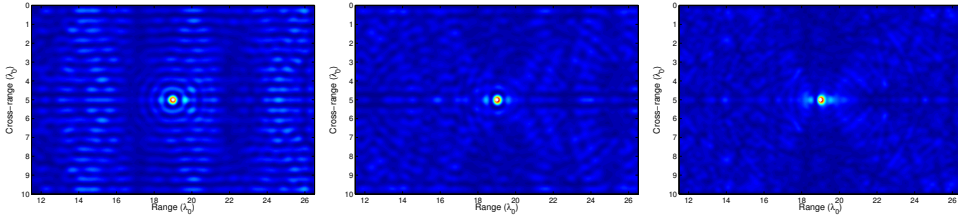
Fig. 10: Imaging with \mathcal{I}^a for multiple frequencies for a point scatterer placed at (z_s, x_s) = (19, 5)\lambda_0 . The central frequency f_c is the same as in Figure 9. Left image: Bandwidth B = 0.15f_c , Middle image: B = 0.51f_c , Right image: B = 0.92f_c .
