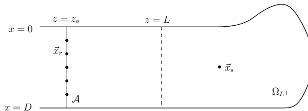
Fig. 2: Passive imaging setup in a terminated waveguide.
