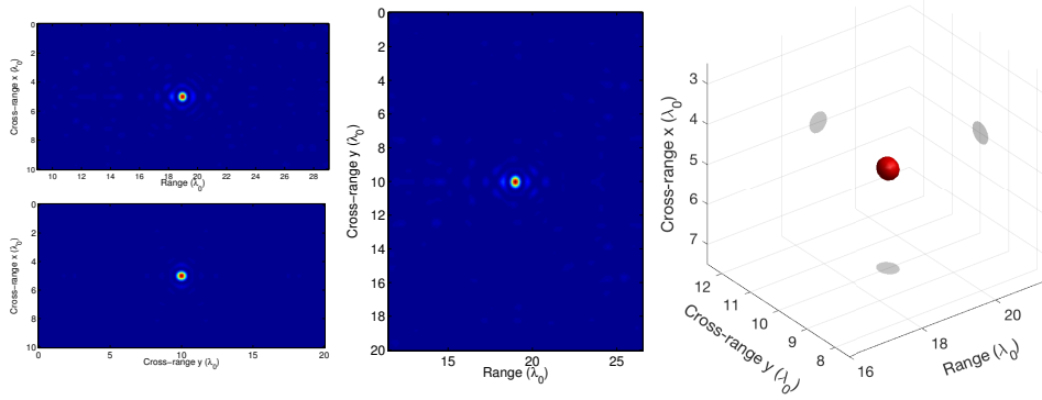
Fig. 21: Modulus of \mathcal{I}^s for the zx -plane (top left), yx -plane (bottom left) and zy -plane (middle), for a single frequency k = 0.973k_0 , k_0 = \pi/10 , for a point reflector placed at \vec{x}^* = (19, 5, 10) \lambda_0 . On the right plot we show the three dimensional reconstruction of the point reflector.
