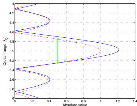
Fig. 6: Comparison between (32) multiplied by 4 (blue line) and J_0(a_x) (red dashed line), for a source located at (z_s, x_s) = (19, 5) \lambda_0 and for a single frequency corresponding to k = 0.973k_0 , where the reference wavenumber is k_0 = \pi/10 . The green arrowed segment indicates length equal to \lambda/2 .
