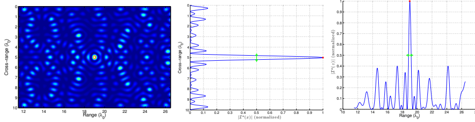
Fig. 5: Normalized modulus of \mathcal{I}^a for a point scatterer located at \vec{x}^* = (19, 5)\lambda_0 and for a single frequency corresponding to k = 0.973k_0 . Imaging on the whole search domain (left), for search points fixed at the correct range z = z^* (middle) and at the correct cross-range x = x^* (right). The green arrowed segment indicates length equal to \lambda/2 and a red asterisk points to the location of the scatterer.
