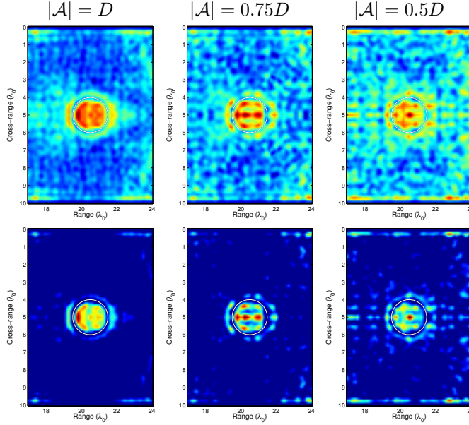
Fig. 19: From left to right: Imaging with \mathcal{I}^a for a disc scatterer centered at (z^*, x^*) = (20.5, 5)\lambda_0 , using a synthetic aperture array with length |\mathcal{A}| = D , 0.75D and 0.5D , for k_c = 0.9733k_0 , k_0 = \pi/10 and B = 0.92f_c . On the top row plots we use no threshold, while for the plots in the bottom row we have a threshold \ell = 0.4 .
