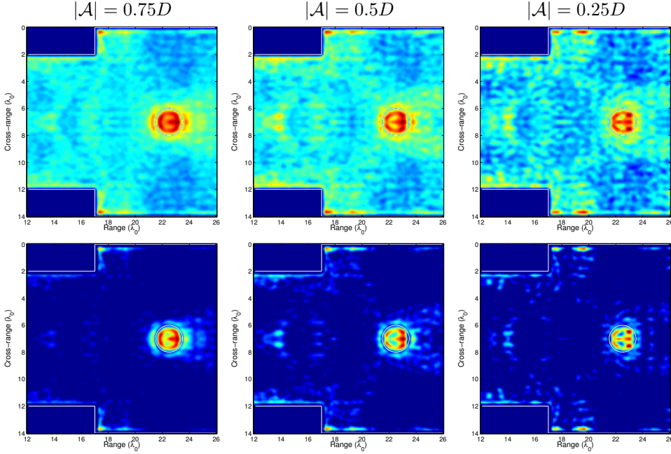
Fig. 17: From left to right: Imaging with \mathcal{I}^a for a disc scatterer centered at (z^*, x^*) = (22.5, 7)\lambda_0 , for different array apertures |\mathcal{A}| = 0.75D , 0.5D and 0.25D , for k_c = 0.9733k_0 , k_0 = \pi/10 and B = 0.92f_c . On the top row plots we use no threshold, while for the plots in the bottom row we have a threshold \ell = 0.4 .
