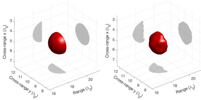
Fig. 23: Imaging a hemisphere with diameter b = 2\lambda_0 , centered at \vec{x}^* = (19, 5, 10)\lambda_0 . The true reflector is shown on the left. The modulus of \mathcal{I}^a for a single frequency k_c = 0.9733k_0 is on the right plot.
