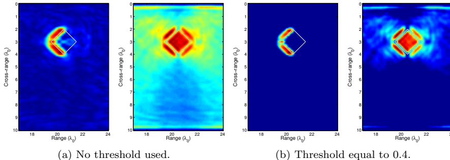
Fig. 14: Imaging with \mathcal{I}^a of a rhombus-shaped scatterer centered at (z^*, x^*) = (20.5, 3)\lambda_0 , for k_c = 0.9733k_0 , k_0 = \pi/10 and B = 0.92f_c . (a) Data are back propagated with the Green’s function for the open ended (left subplot) and the terminating waveguide (right subplot), where we do not use thresholding. (b) Same setup as in (a) but we use thresholding with \ell = 0.4 .
