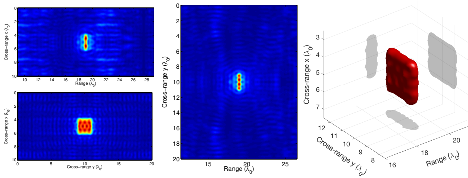
Fig. 22: Modulus of \mathcal{I}^s for the zx -plane (top left), yx -plane (bottom left) and zy -plane (middle), for a single frequency k = 0.973k_0 for a square reflector [9, 11]\lambda_0 \times [4, 6]\lambda_0 placed at z = 19\lambda_0 . On the right plot we show the three dimensional reconstruction of the square reflector.
