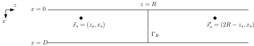
Fig. 24: Two sources placed symmetrically with respect to \Gamma_R
