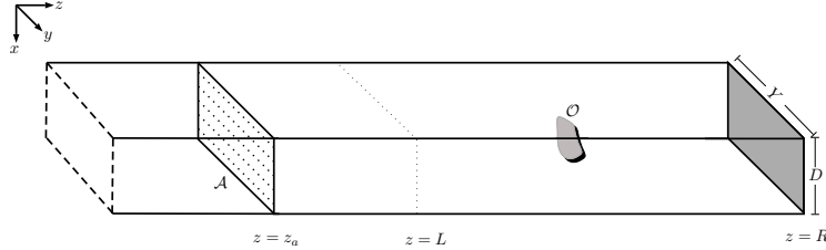
Fig. 20: Schematic representation of the imaging setup in a three-dimensional waveguide.
